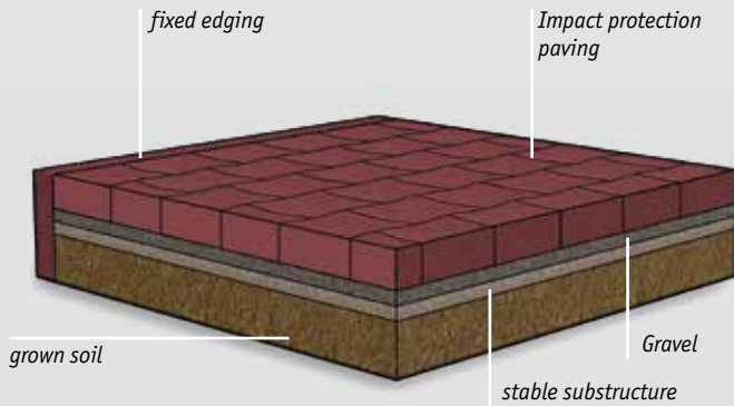
Laying the Terrasoft paving stones on a permeable substrate (not vehicle load-bearing).
